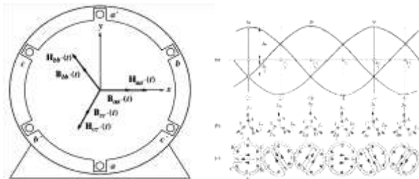
Figure 3. magnetic field intensity vectors H(t) (MFD vector B(t) ) produced by each coil
