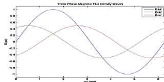
Figure 6. The sine, cosine and the net sinusoidal waves of magnetic field density
