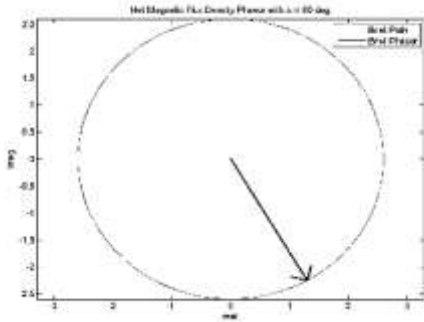
Figure 11. Rotating magnetic field in case of a split-phase with angle of 60°.
